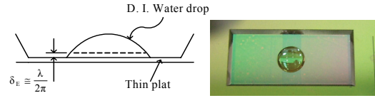
Figure 4 The liquid droplet on the FPW device
