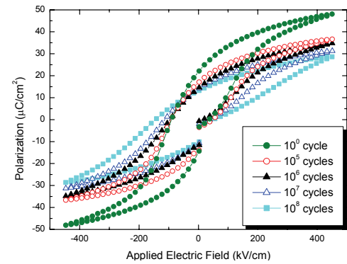
Figure 7 The fatigue characteristics for the PZT film with LSMO buffer layer
