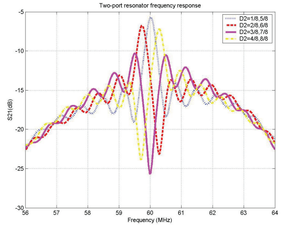
Figure 3 Two-port SAW resonator frequency response
