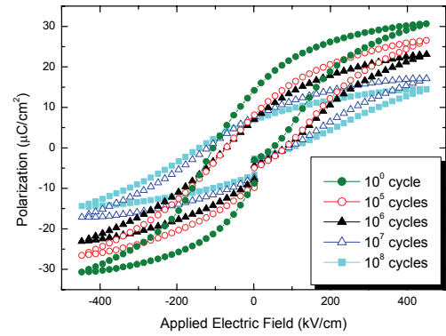
Figure 6 The fatigue characteristics for the PZT film without LSMO buffer layer
