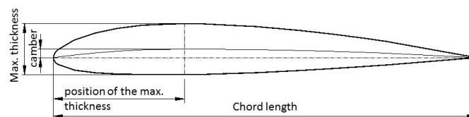
Figure 1. The NACA Profile geometry.
